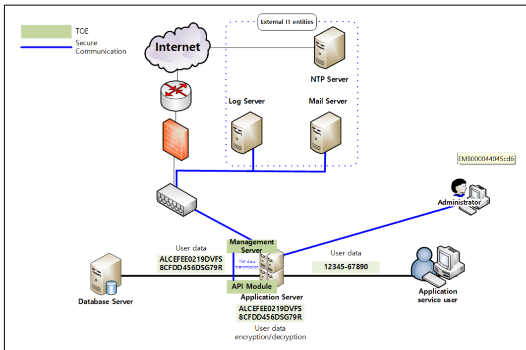
[Figure 4] Operational environment of Database Encryption (4)
